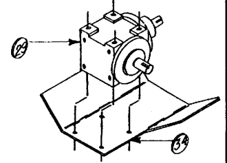
DETAILED VIEW OF PTO GEAR BOX
