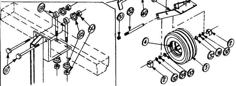
TYPICAL MOUNTING HARDWARE FOR 6x4 TOOL BAR
