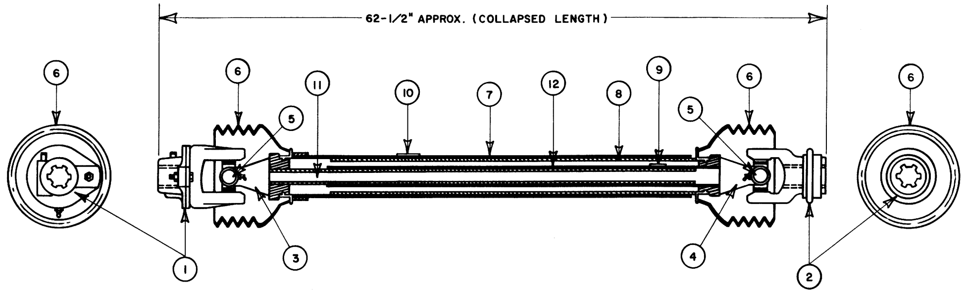
MODEL 94 PTO GEAR BOX TO CHAIN CASE DRIVELINE
