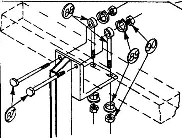
TYPICAL MOUNTING HARDWARE FOR 6x4 TOOL BAR
