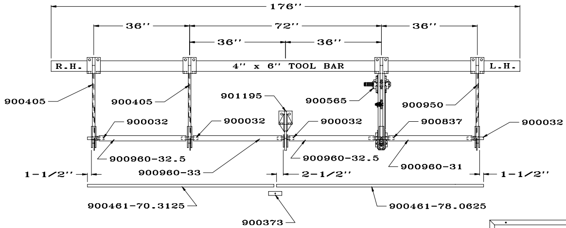
4 ROW-36 SHANK LAYOUT
