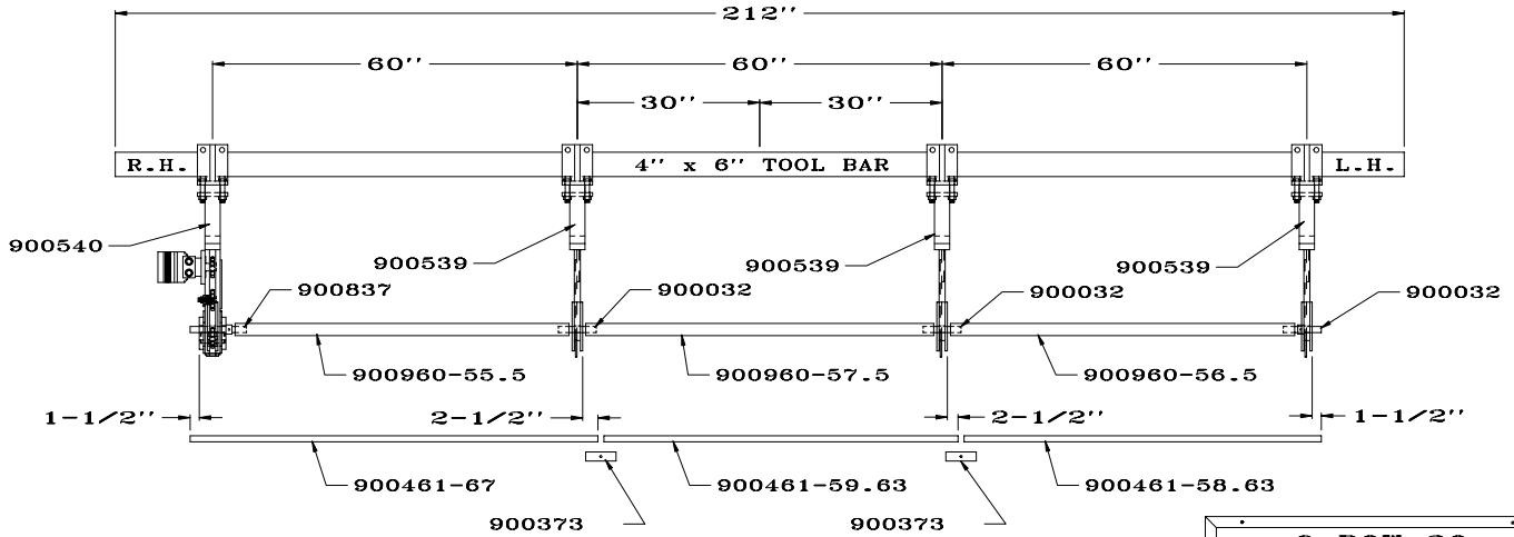
6 ROW-30 C-SHANK LAYOUT
