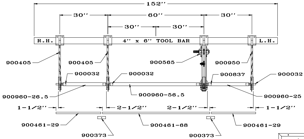
4 ROW-30 SHANK LAYOUT
