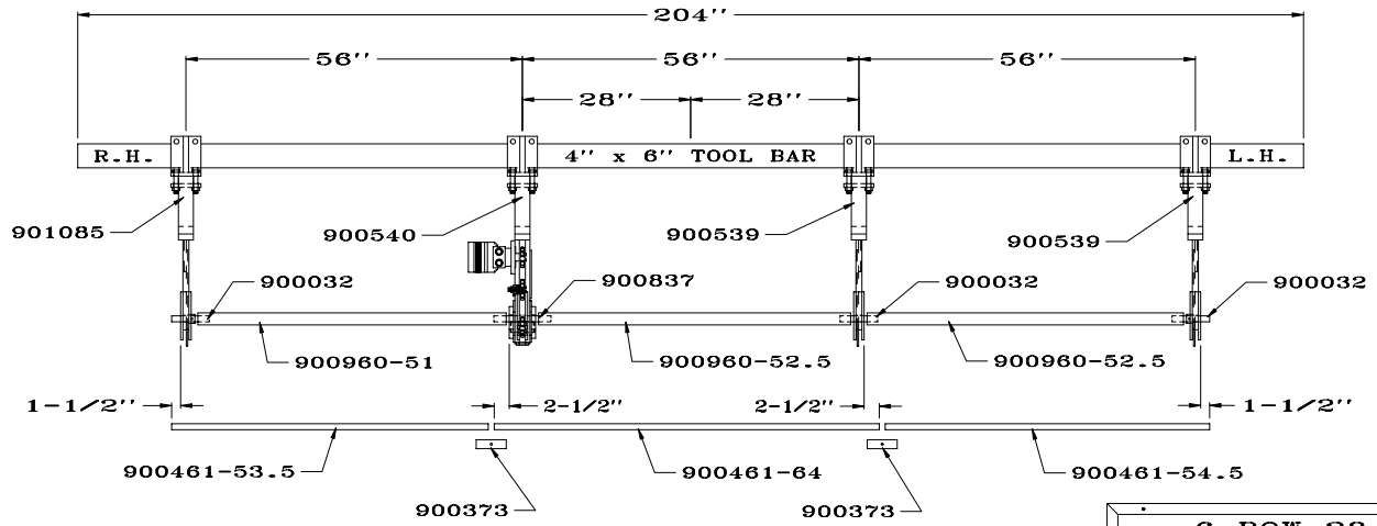
6 ROW-28 C-SHANK LAYOUT
