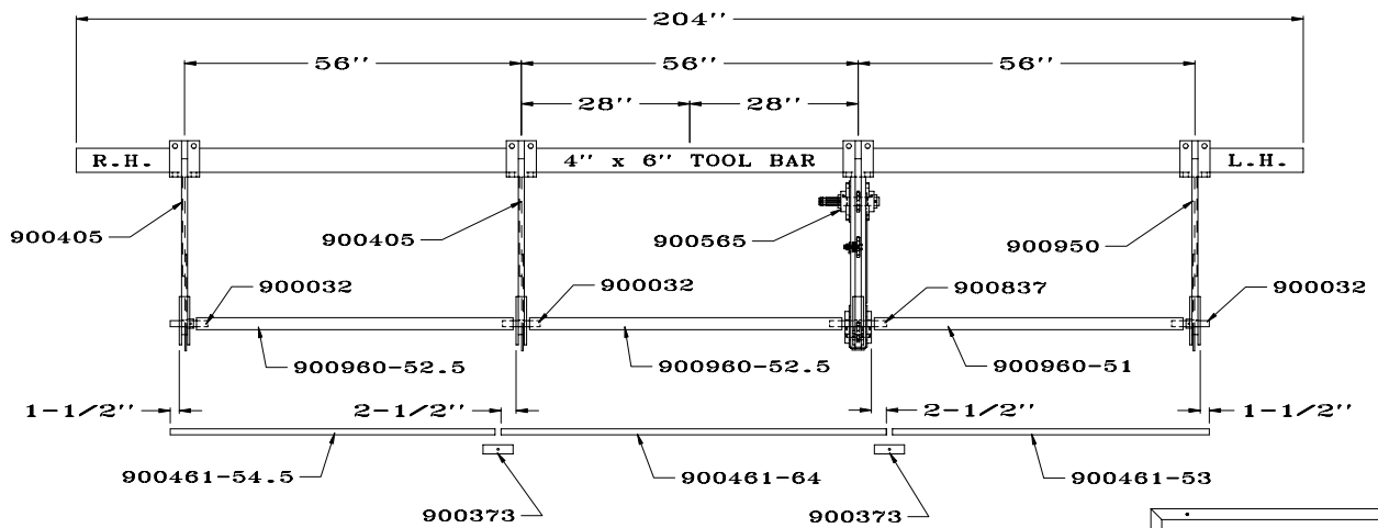
6 ROW-28 SHANK LAYOUT
